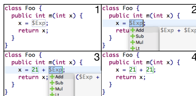
Figure 1. (1) Incomplete program with explicit placeholders. (2) Triggering completion for a placeholder. (3) After selecting a proposal, showing completions for nested placeholders. (4) Completing a nested placeholder by typing.
